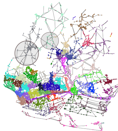
Figure 1: Road network clustering
